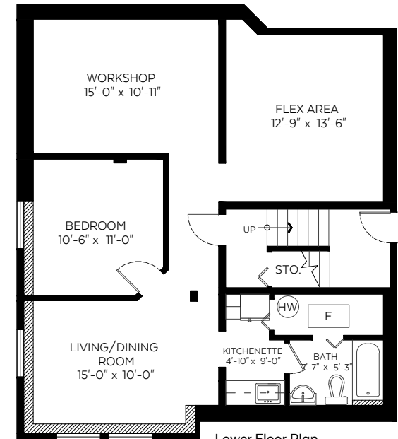
Lower Floor Plan Floor Area: 1,037 sq.ft. Ceiling Height: 8 ft.
