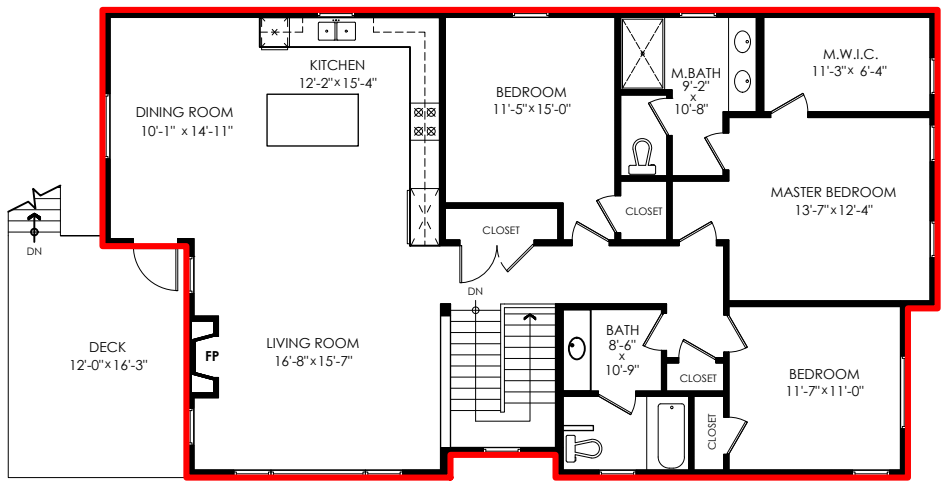
Upper Floor Plan Floor Area: 1650 sq.ft. Ceiling Height: 8'-11"
