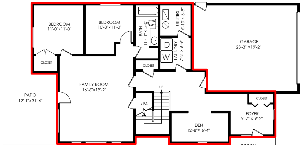
Main Floor Plan Floor Area: 1246 sq.ft. Ceiling Height: 8'-11"
