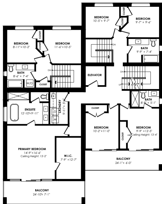
Upper Floor Plan Floor Area: 2298 sq.ft. Ceiling Height: 9'
